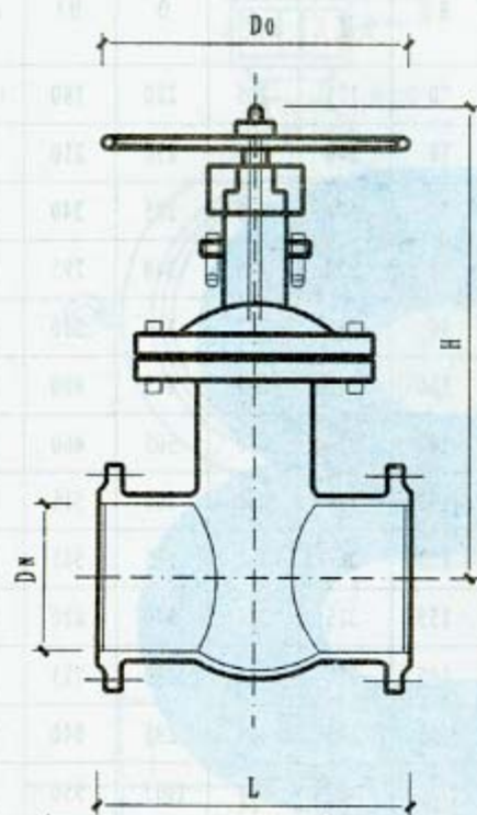
闸阀
